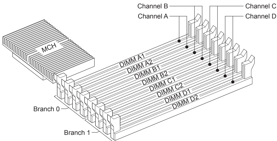
Figure 11. Memory Layout
