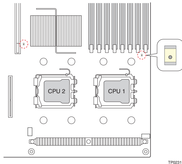
Figure 23. Processor Fault LED Location
