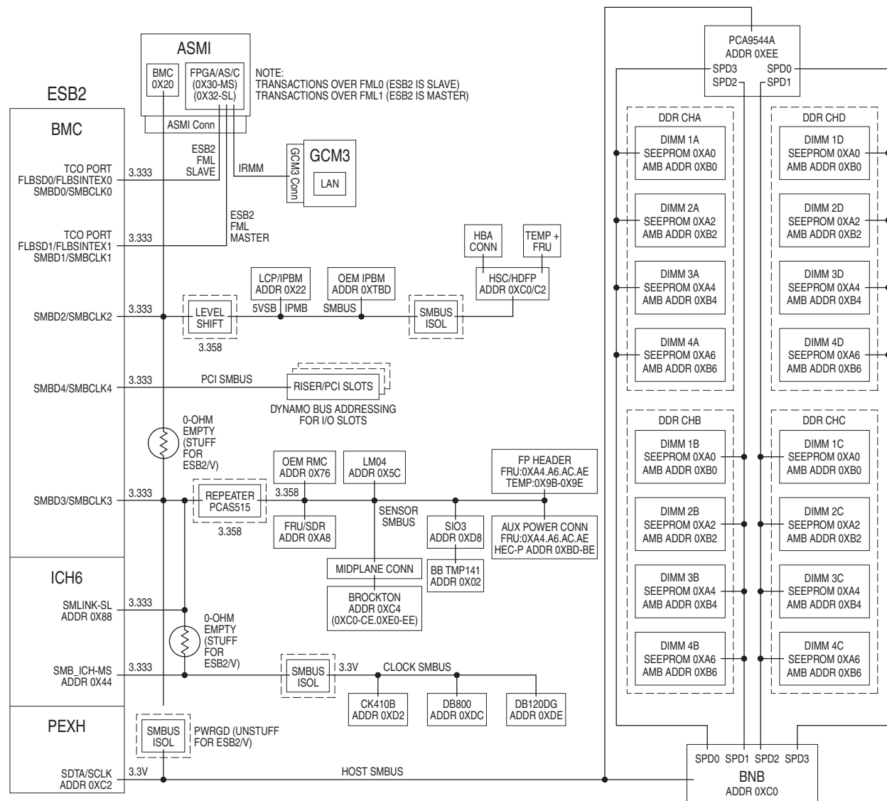
Figure 16. SMBUS Block Diagram
