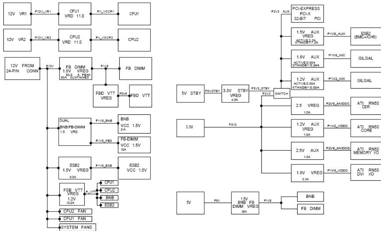
Figure 25. Power Distribution Block Diagram
